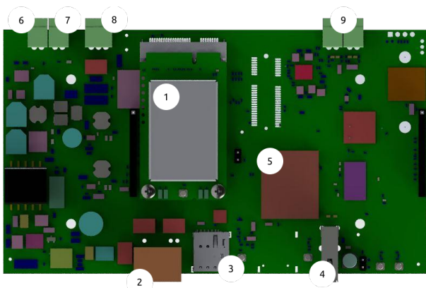
Figure 5: MainBoard
