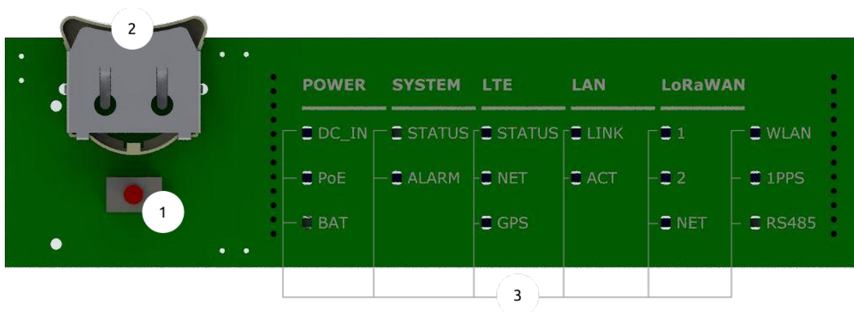
Figure 6: Indication Board
