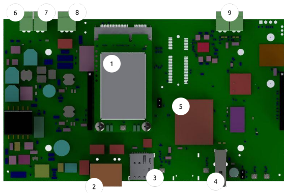
Figure 4: Mainboard
