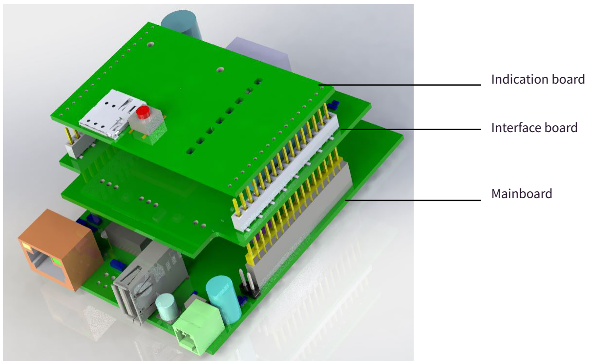
Figure 1: Triple control module (model 501 EU is shown)
